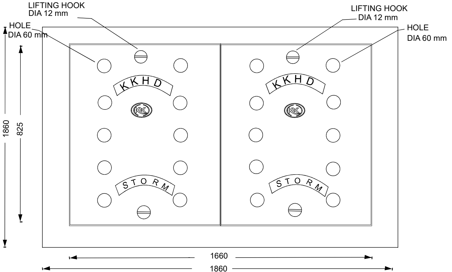
PLAN
