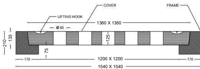
DETAILED SECTION AA
