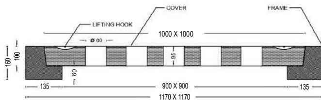
DETAILED SECTION AA
