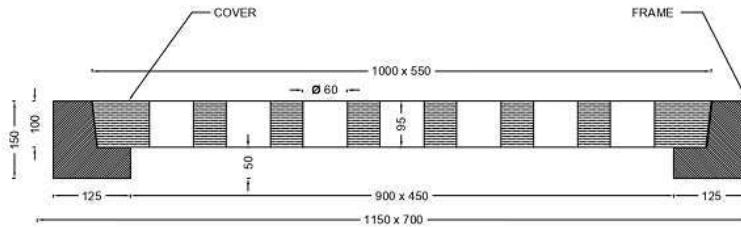
DETAILED SECTION AA
