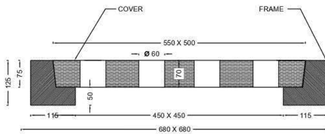
DETAILED SECTION AA
