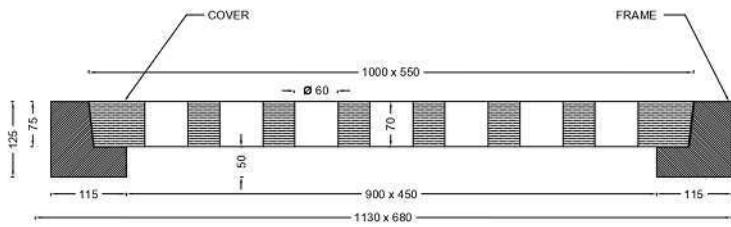
DETAILED SECTION AA
