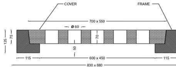
DETAILED SECTION AA
