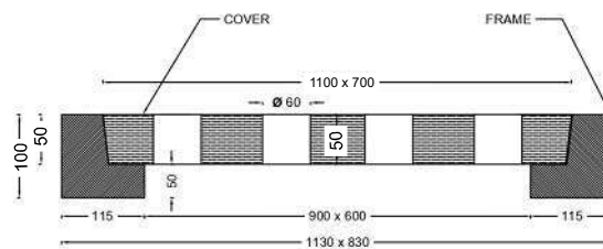
DETAILED SECTION AA
