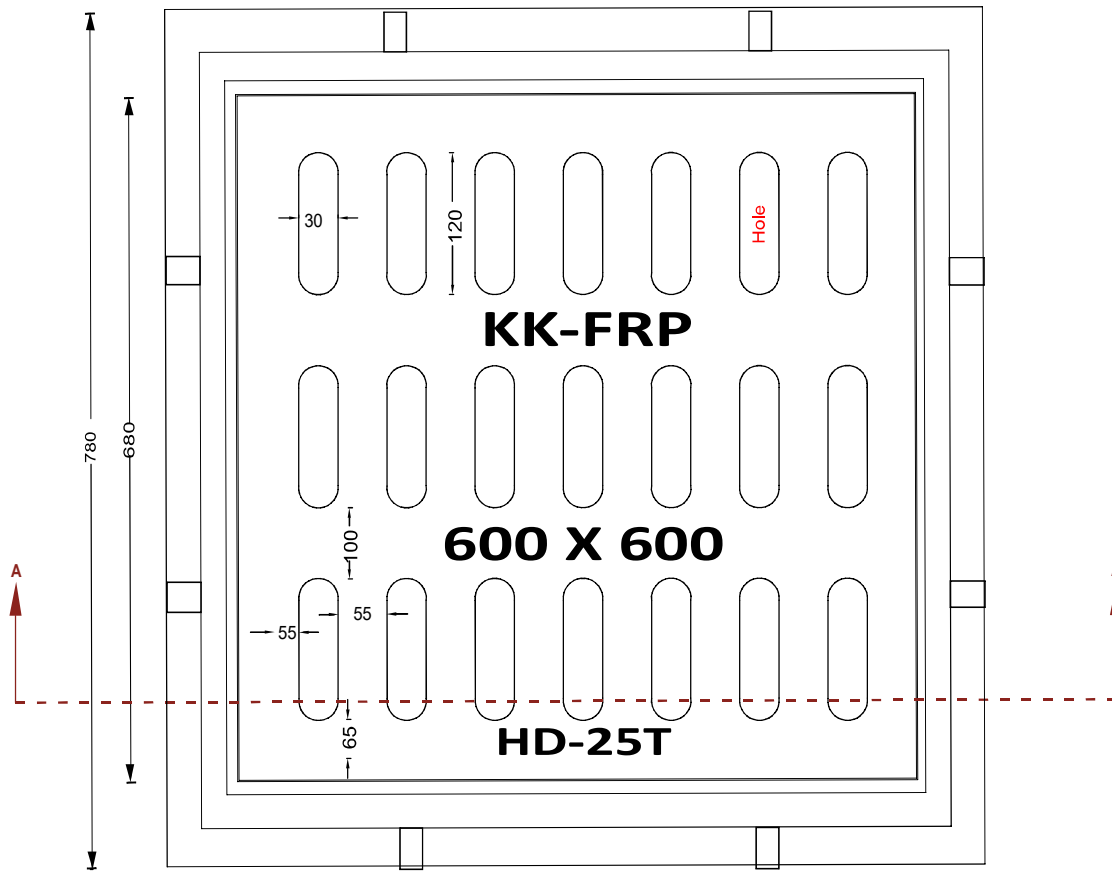
PLAN
