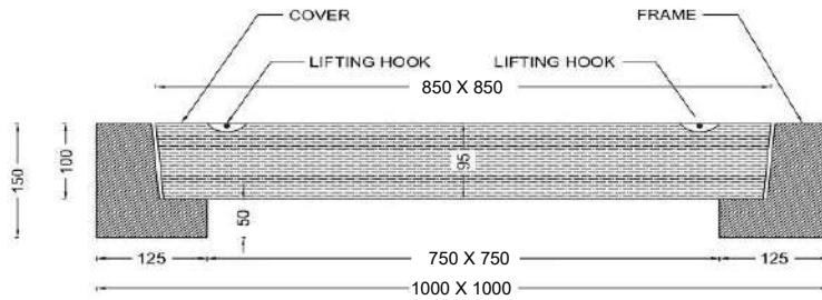
DETAILED SECTION AA
