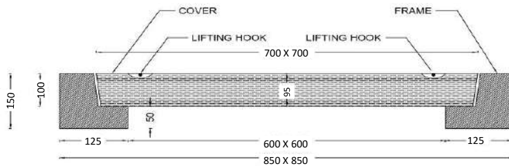
DETAILED SECTION AA
