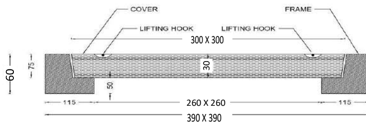
DETAILED SECTION AA
