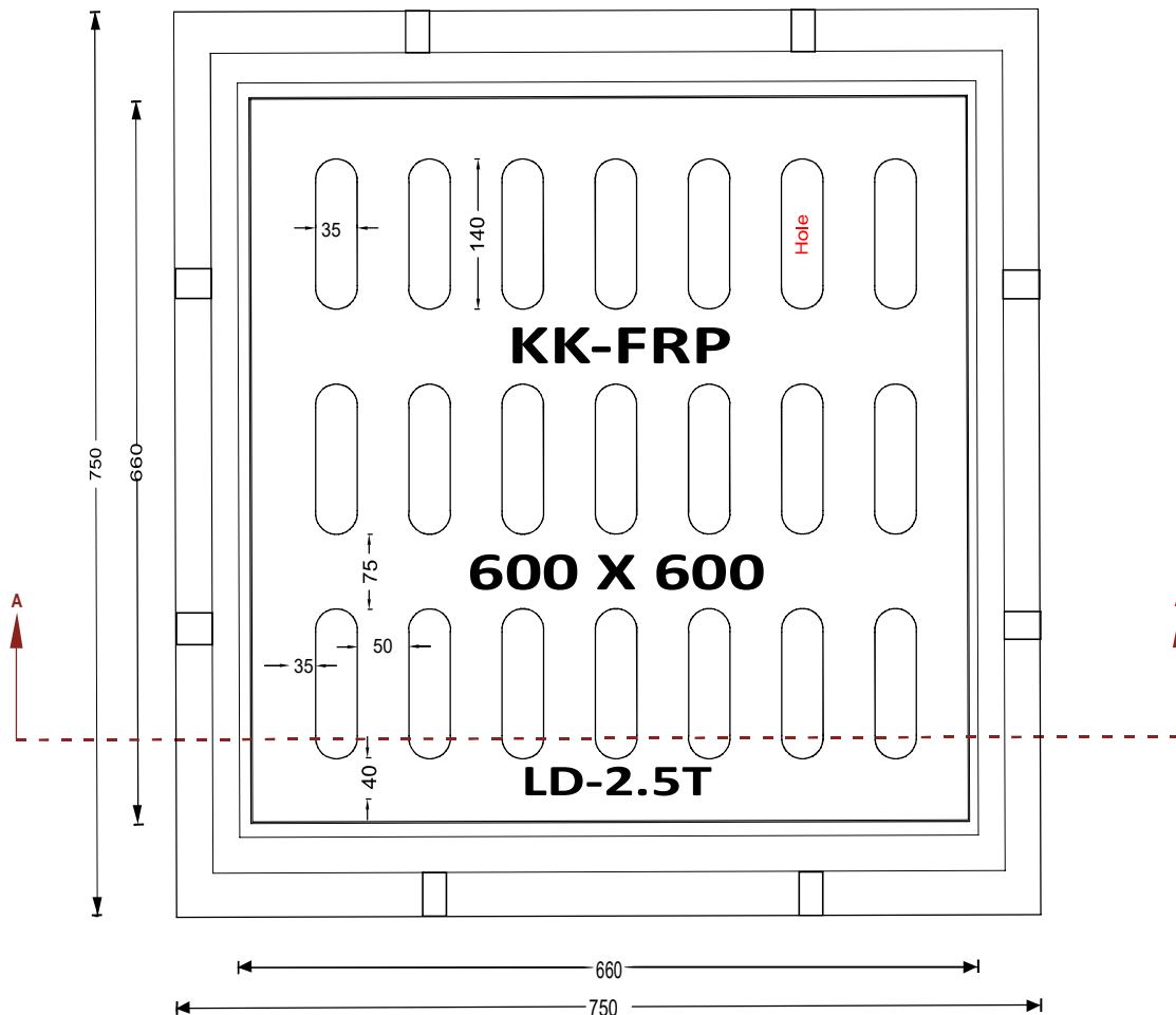
PLAN
