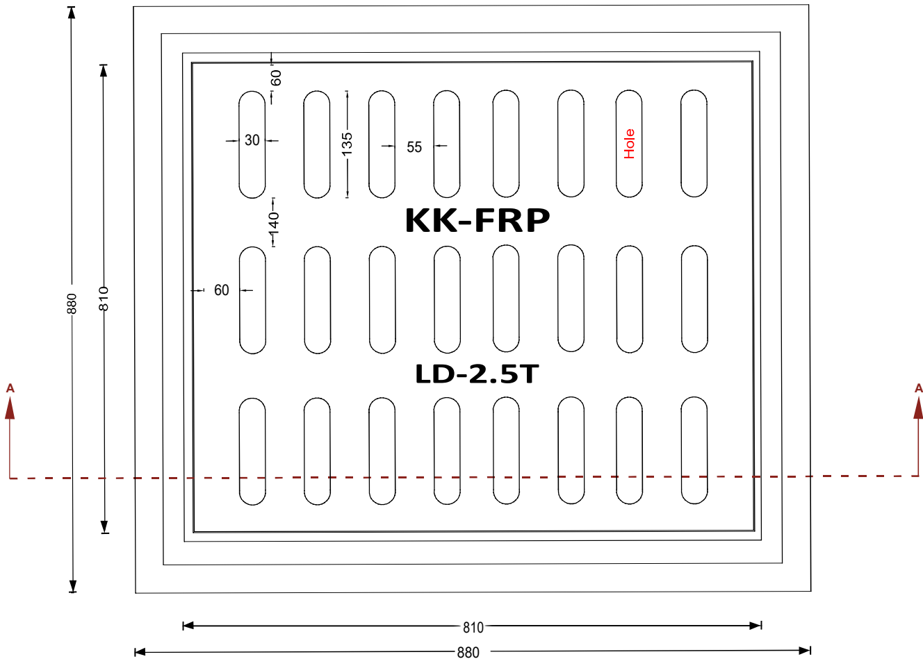
PLAN
