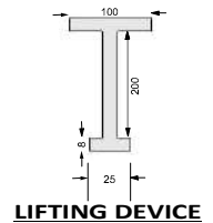
LIFTING DEVICE
