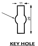
KEY HOLE
