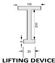
LIFTING DEVICE
