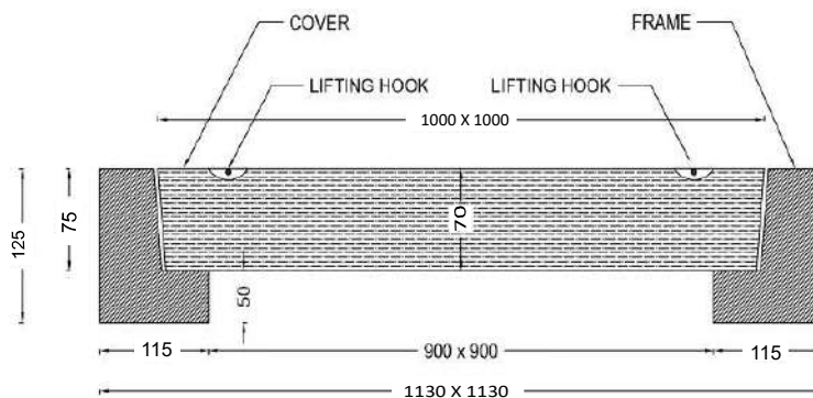
DETAILED SECTION AA
